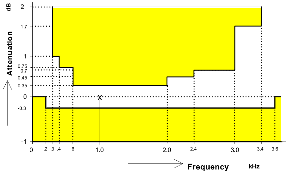
Figure 25 Frequency Response Receive
