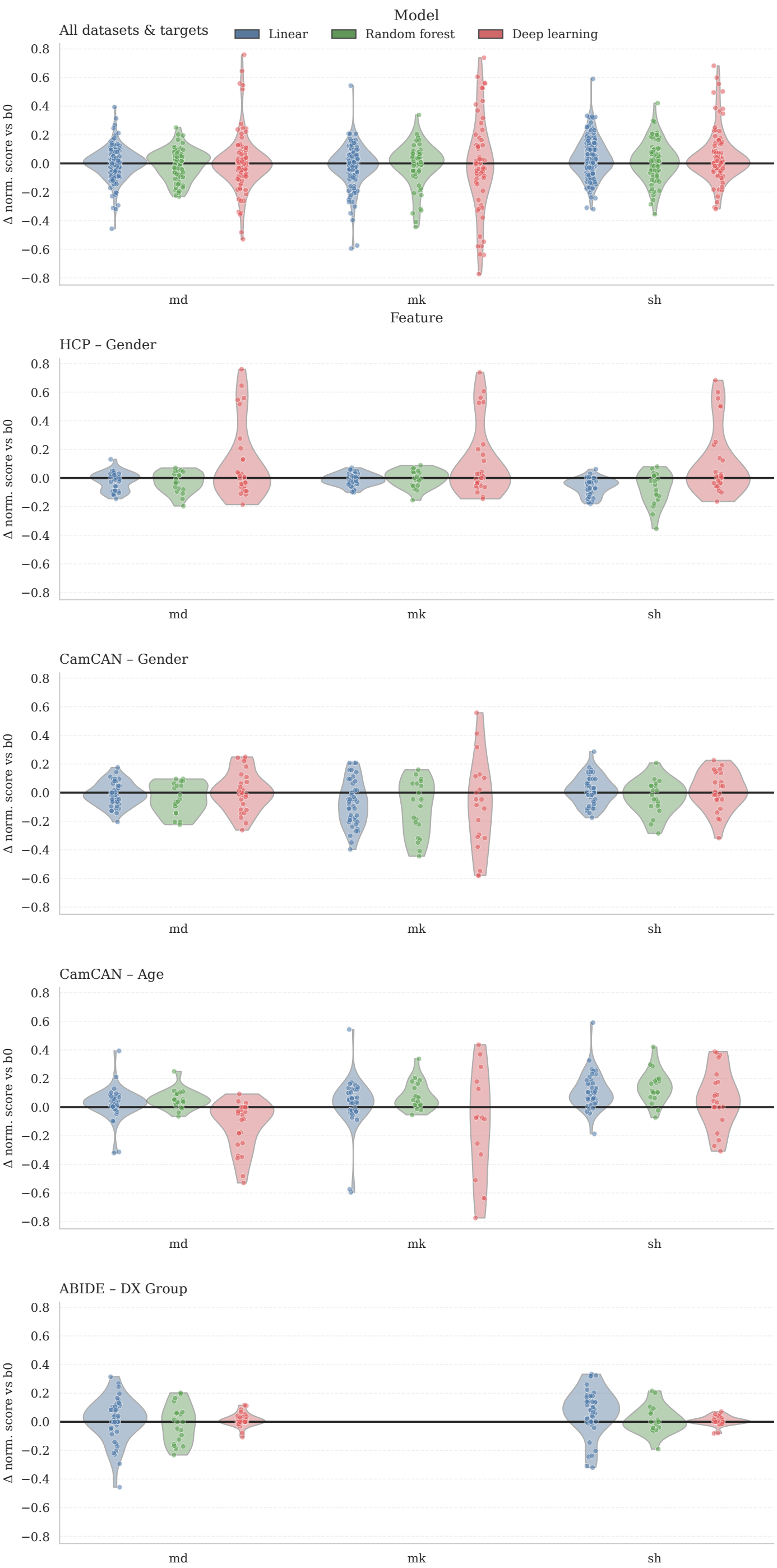
Feature benefit vs b0 by model (paired \Delta normalized score)
