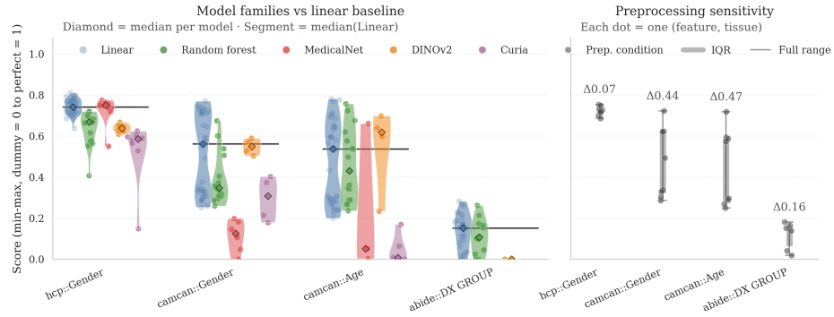
Fig. 2. Summary of benchmark results across datasets, feature representations and models.
