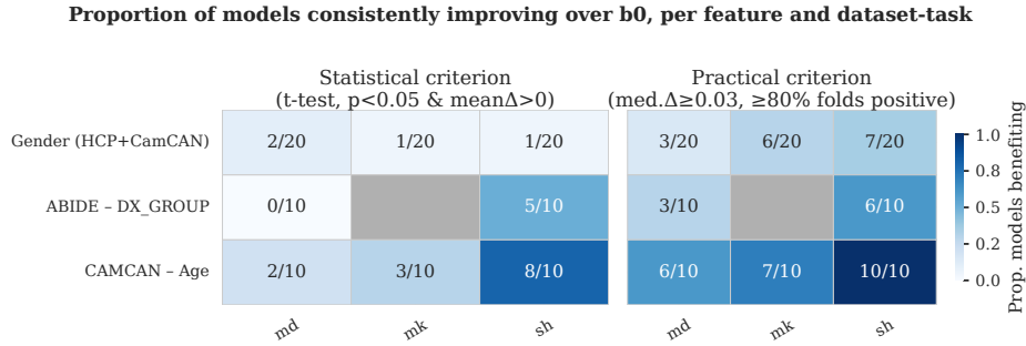
Fig. 5. Proportion of models improving over the non-diffusion baseline (b0), stratified by task and feature. Improvement is based on fold-level normalized differences ( \Delta = \text{feature} - \text{b0} ). Left: statistical criterion (t-test against zero, p < 0.05 and \text{mean}\Delta > 0 ); Right: robustness criterion (median \Delta \geq 0.03 and \geq 80\% positive folds). Cells report the fraction of models meeting each criterion per target (rows) and feature (columns).
