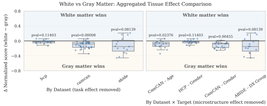
Fig. 4. Fold-level paired comparison of white vs. gray matter using normalized scores ( 0 = \text{dummy} , 1 = \text{perfect} ). Each point shows the matched fold difference ( \Delta = \text{white} - \text{gray} ) under identical settings. Left: dataset-level tissue effects; Right: task-level effects. Boxplots summarize fold differences; p-values test mean effects against zero.
