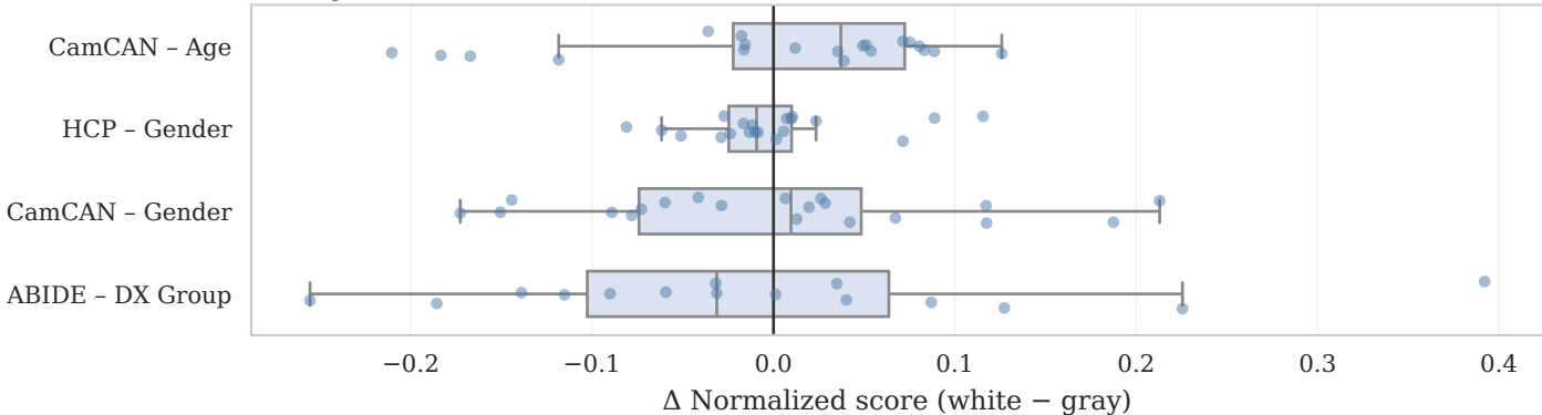
White vs Gray Matter: Task Tissue Effect (Dataset-Feature Baseline Removed) Gray matter wins White matter wins
