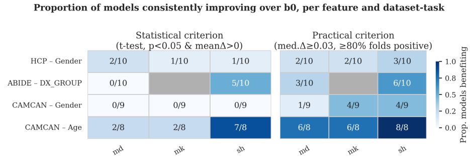
Fig. 4. Impact of different feature representations on prediction performance across datasets and tasks.
