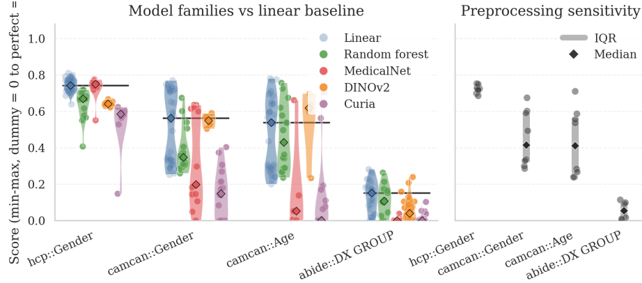
Fig. 2. Summary of benchmark results across datasets, feature representations and models.
