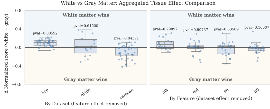
Fig. 3. Comparison of white vs gray matter performance across datasets and feature representations.
