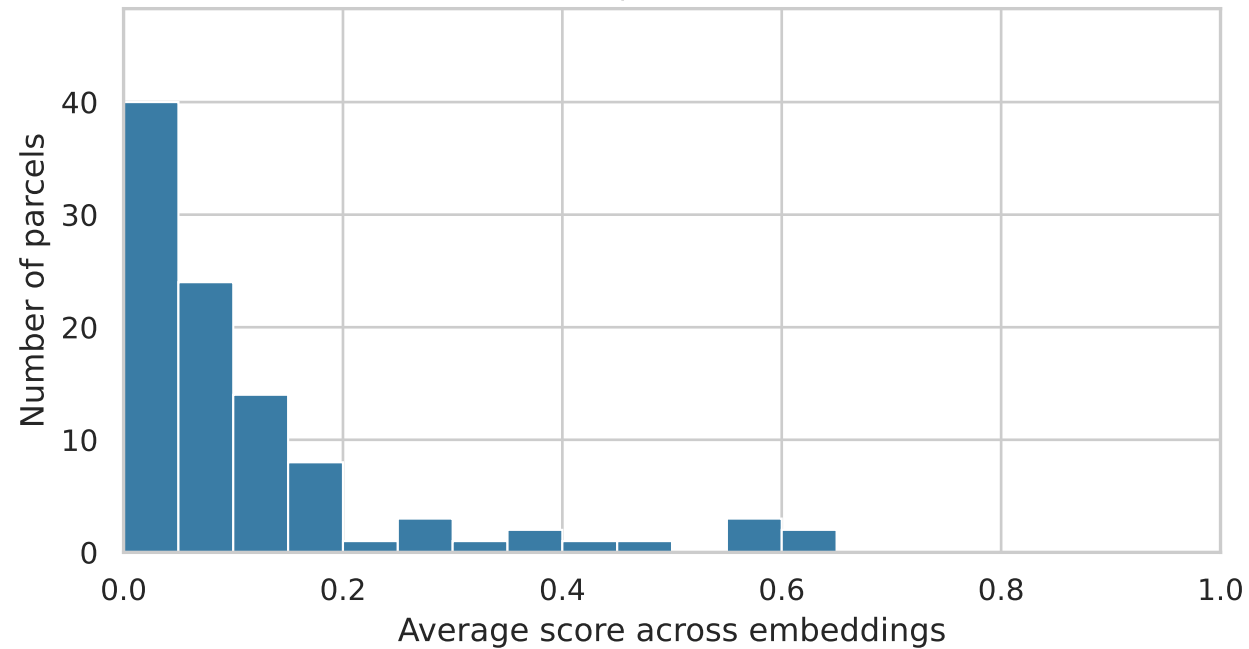
hcp | Elasticnet
