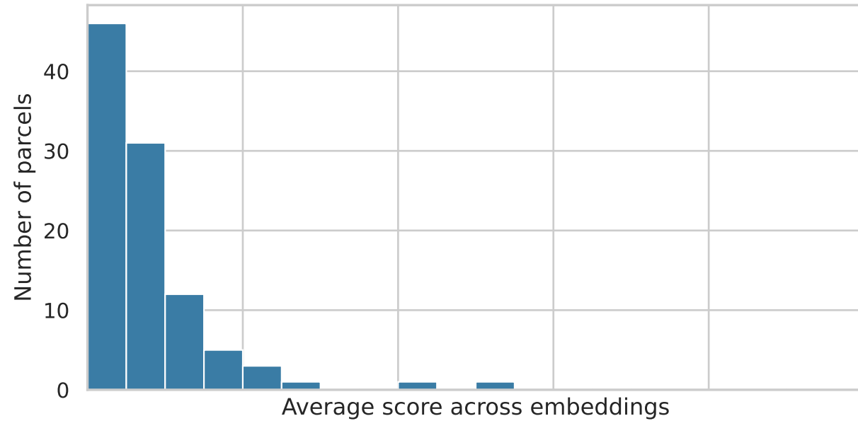
camcan | Elasticnet
