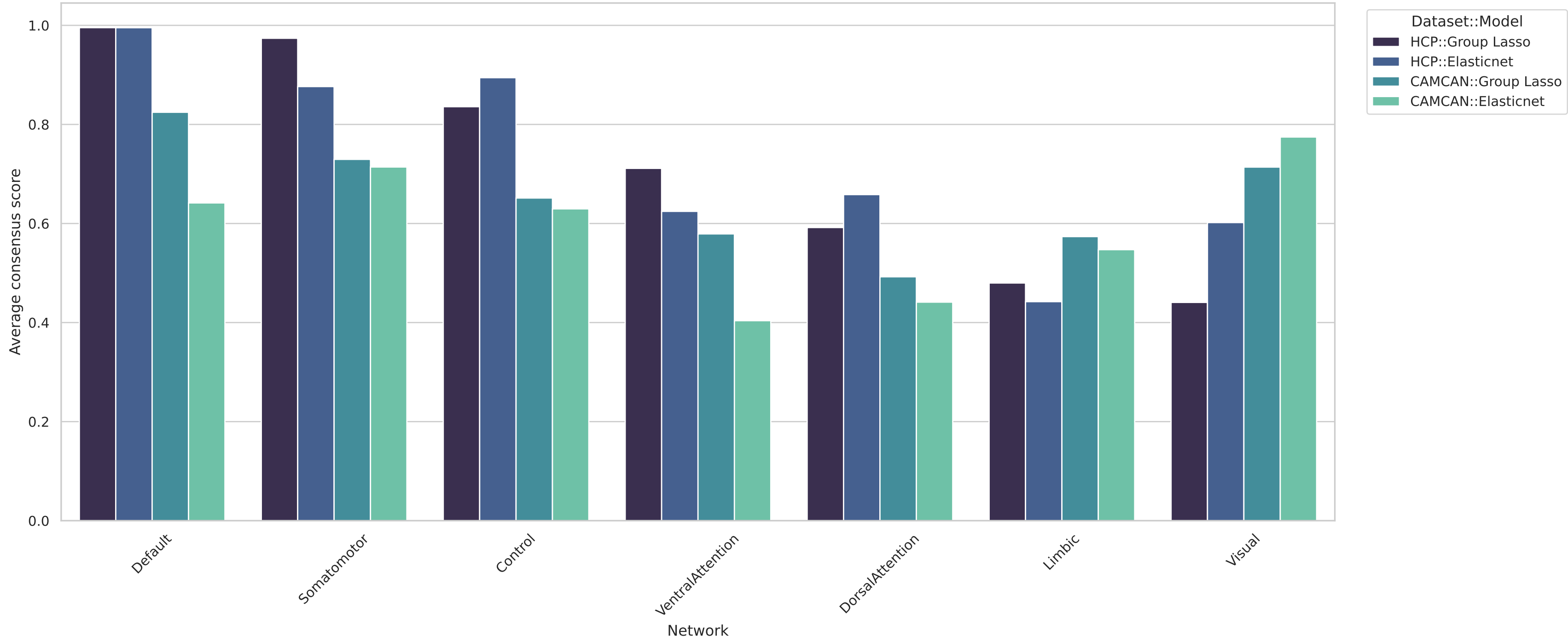
Network consensus scores by dataset and model Ordered by HCP::Group Lasso | binary_classification | md | embeddings: flatten, summary_stats, mean_std, percentiles, pca
