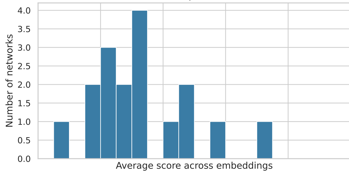
camcan | Elasticnet
