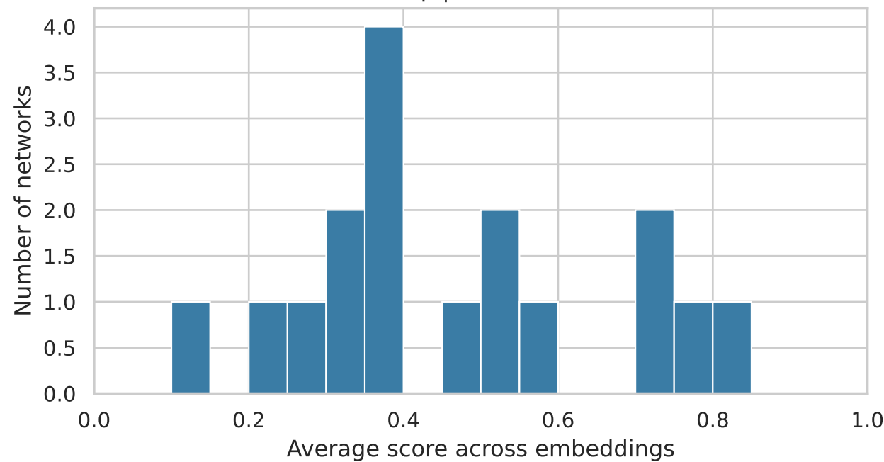
hcp | Elasticnet
