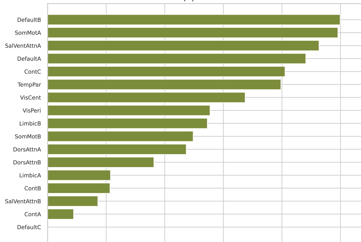
hcp | Elasticnet
