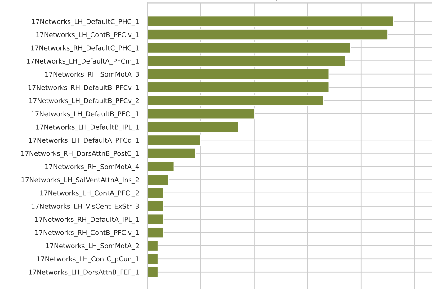
hcp | Elasticnet
