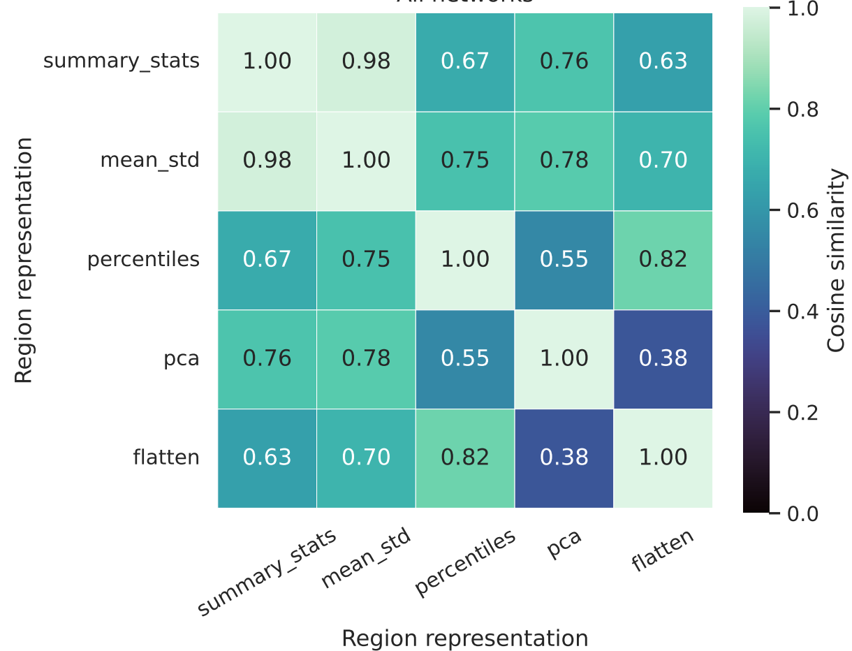
All networks
