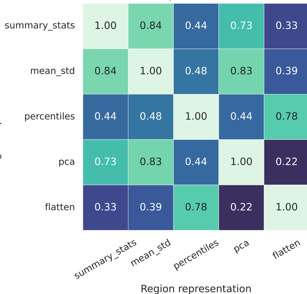
Top 5 networks
