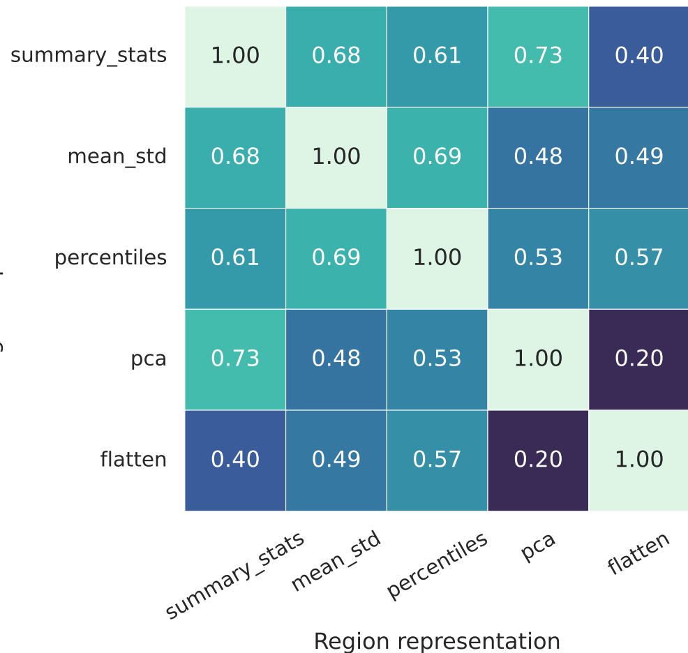
Top 5 networks
