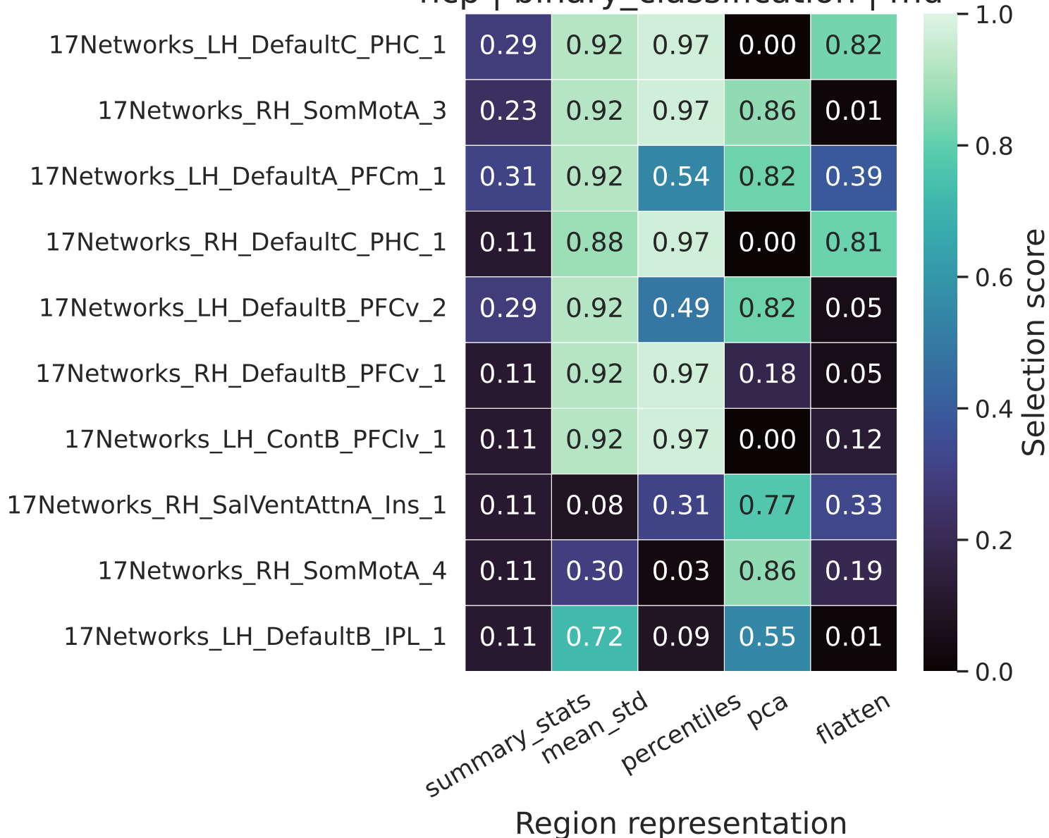
Top 10 selected regions - Elasticnet hcp | binary_classification | md
