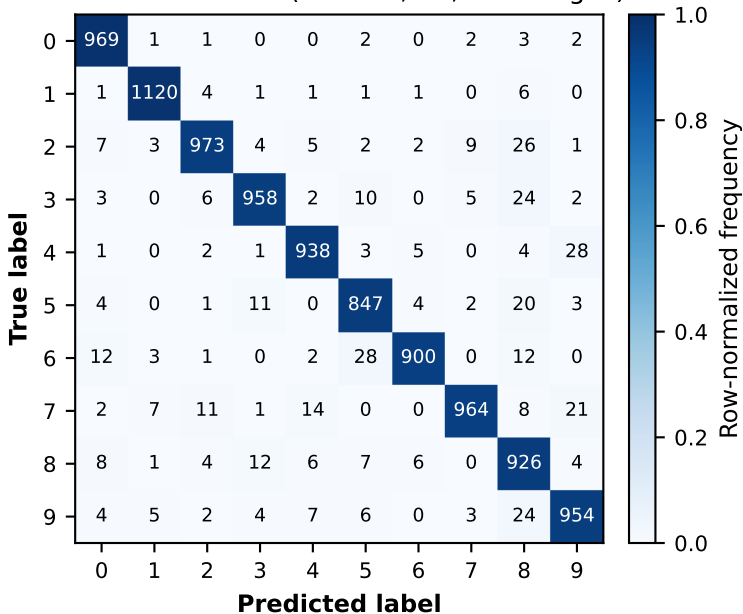
Confusion matrix (test set, 10,000 images)
