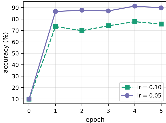
(b) Test accuracy
