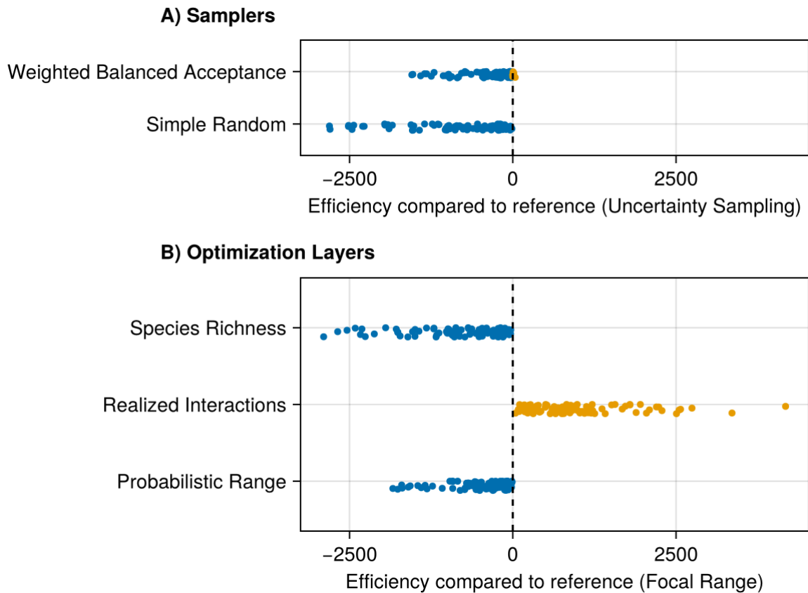
202 203 Figure 5: Within-simulation comparison of efficiency between samplers and optimization layers. The 204 comparison values is based on the difference of the definite integrals of the efficiency samplers curves 205 described in Equation 3. Negative values (in blue) indicate that the compared option lead to a less efficient 206 sampling than its reference, while positive values (in orange) indicate it was more efficient. References were 207 chosen for narrative purposes and to simplify the number of comparisons displayed. All one-by-one 208 comparisons are available in Supp. Mat.
