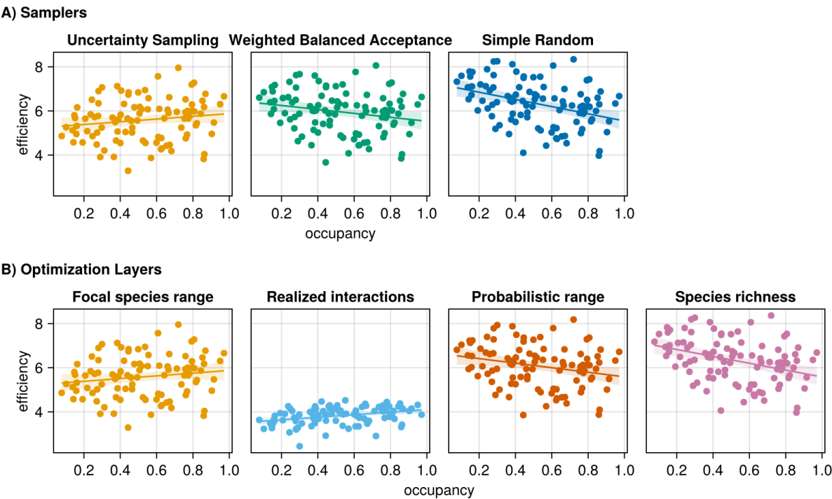
230 231 Figure 6: Relationship between the occupancy of the focal species and sampling efficiency for all optimization 232 options. These results come from 100 independent simulations, and therefore 100 different sets of metawebs, 233 species ranges, and occupancy of the focal species.
