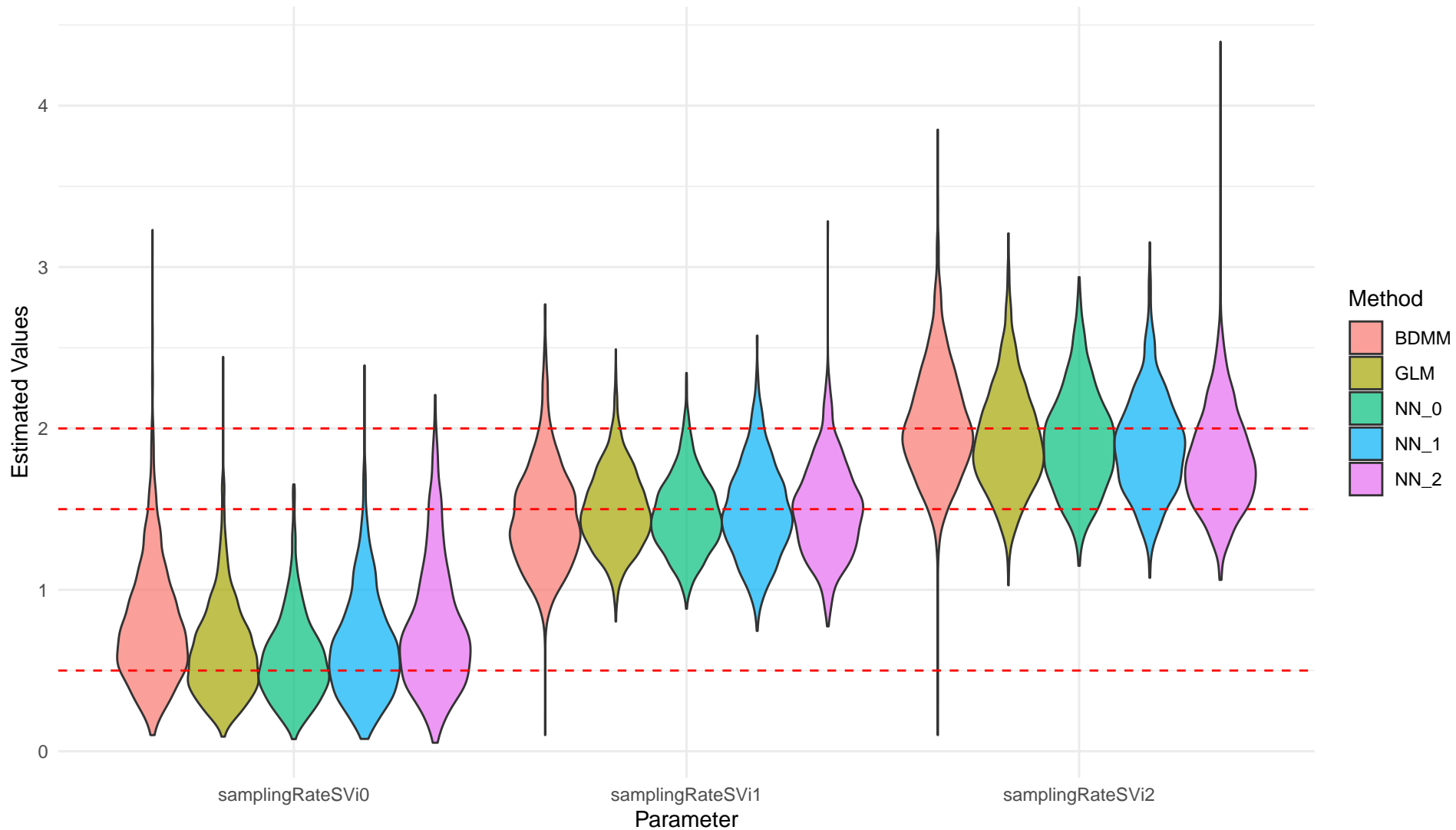
Comparison of Posterior Distributions for Different Methods
