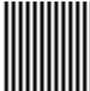
k_x=12.5, k_y=0
