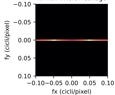
k_x non intero: leakage
