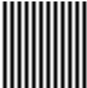
k_x=12, k_y=0
