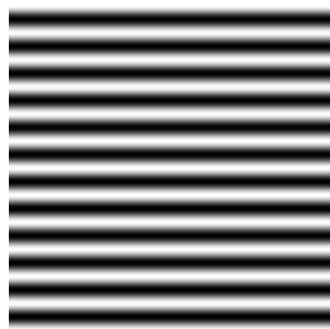
k_x=0, k_y=12
