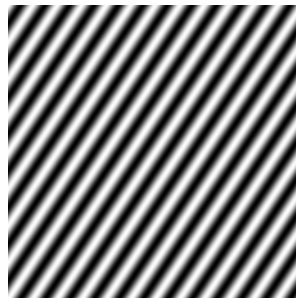
k_x=12, k_y=8
