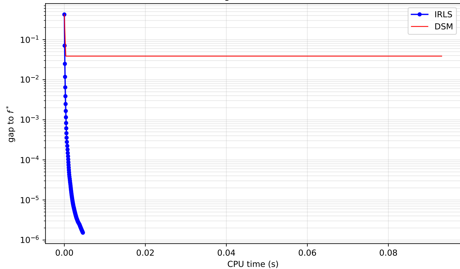
Convergence vs CPU time
