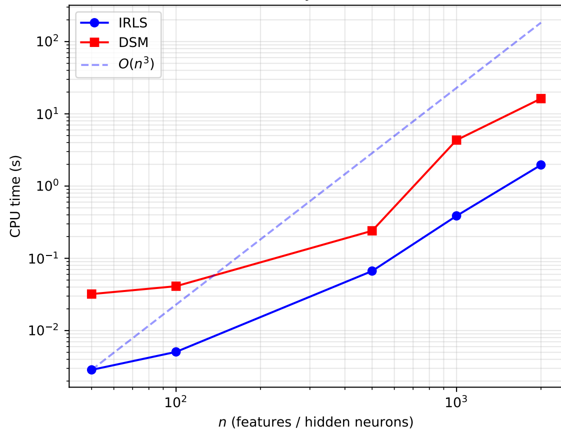
Scalability: total time
