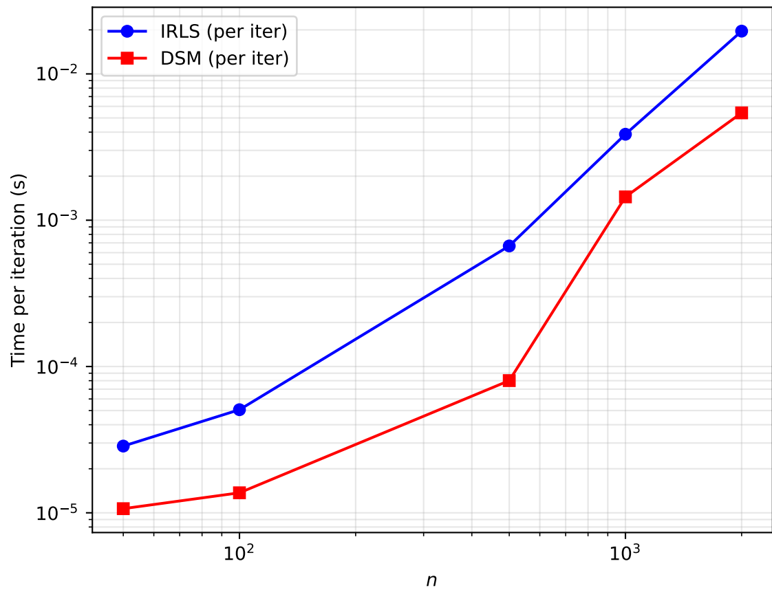
Per-iteration cost
