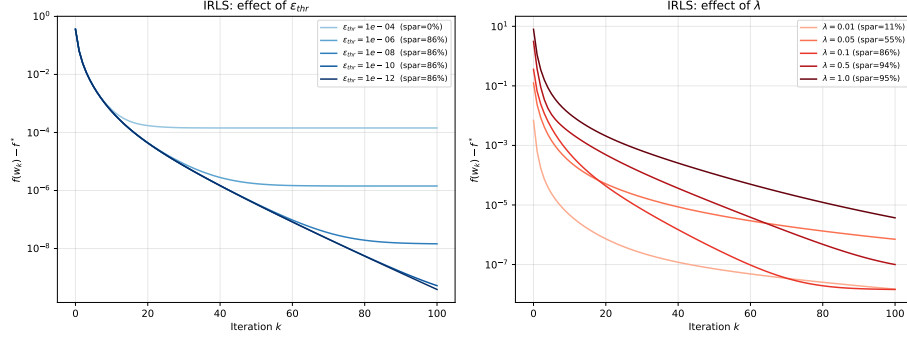
Figure 5.4: IRLS sensitivity. Left: effect of \varepsilon_{thr} on convergence and sparsity at \lambda_{LASSO} = 0.1 . Right: effect of \lambda_{LASSO} at \varepsilon_{thr} = 10^{-8} .
