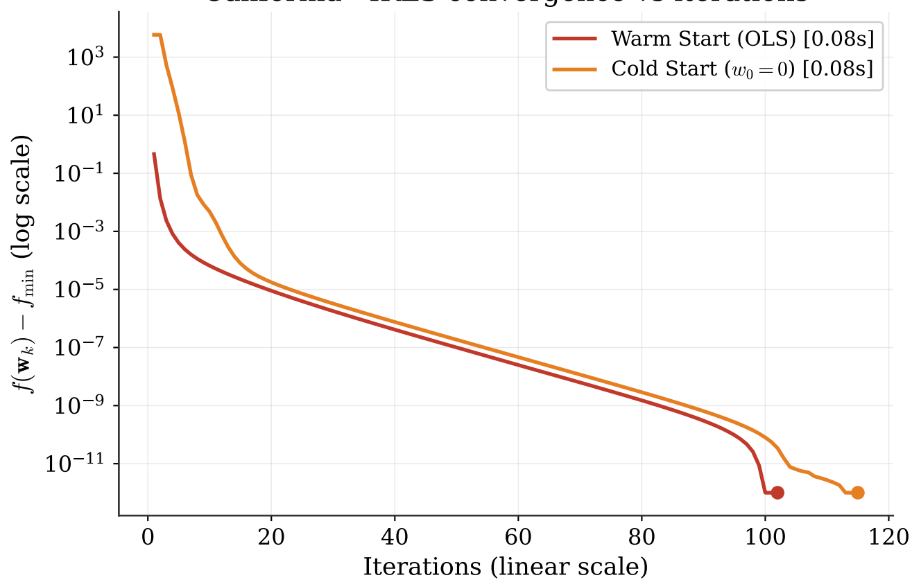
California - IRLS convergence vs iterations
