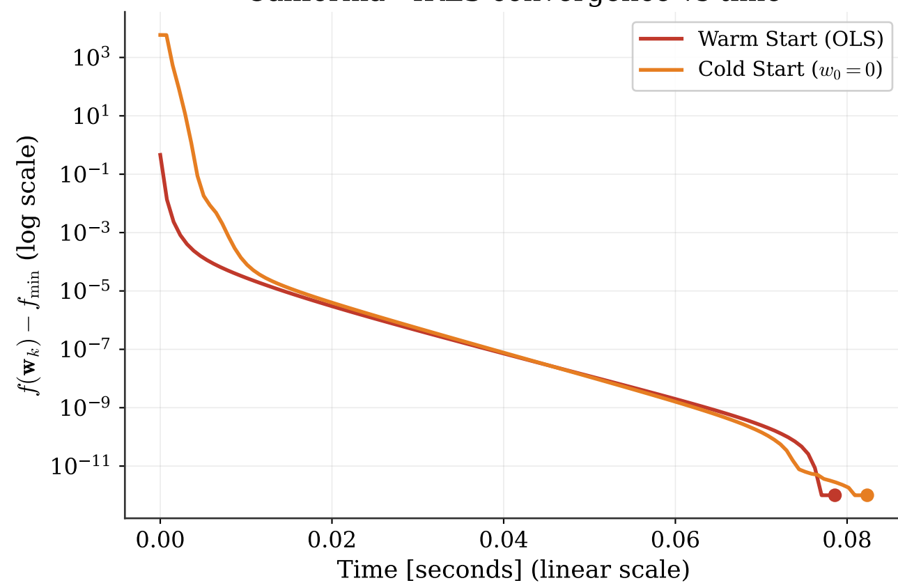
California - IRLS convergence vs time
