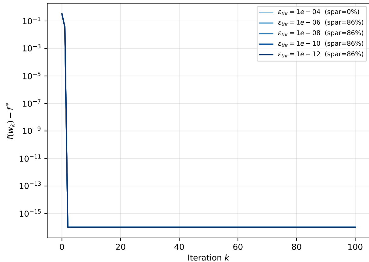
IRLS: effect of \varepsilon_{thr}
