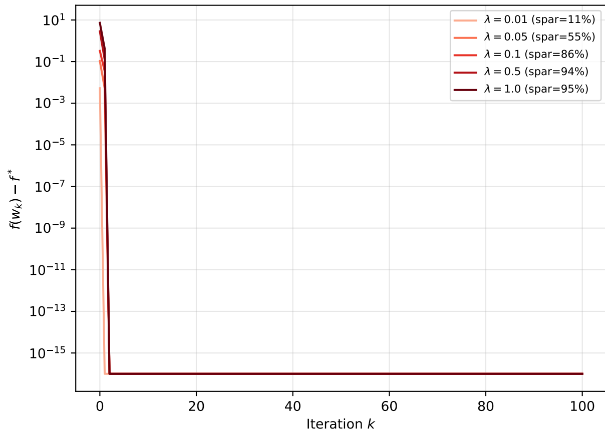
IRLS: effect of \lambda
