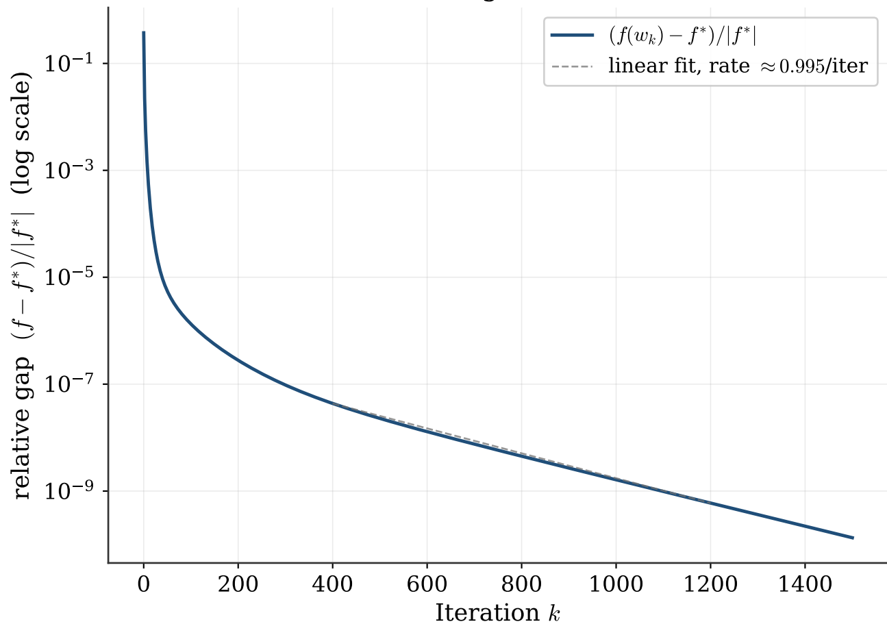
IRLS: linear convergence (slow, rate \approx 1 )
