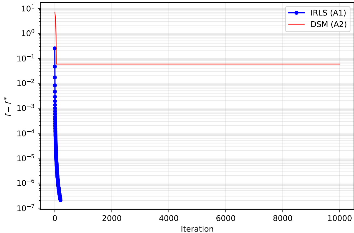
Convergence vs iterations
