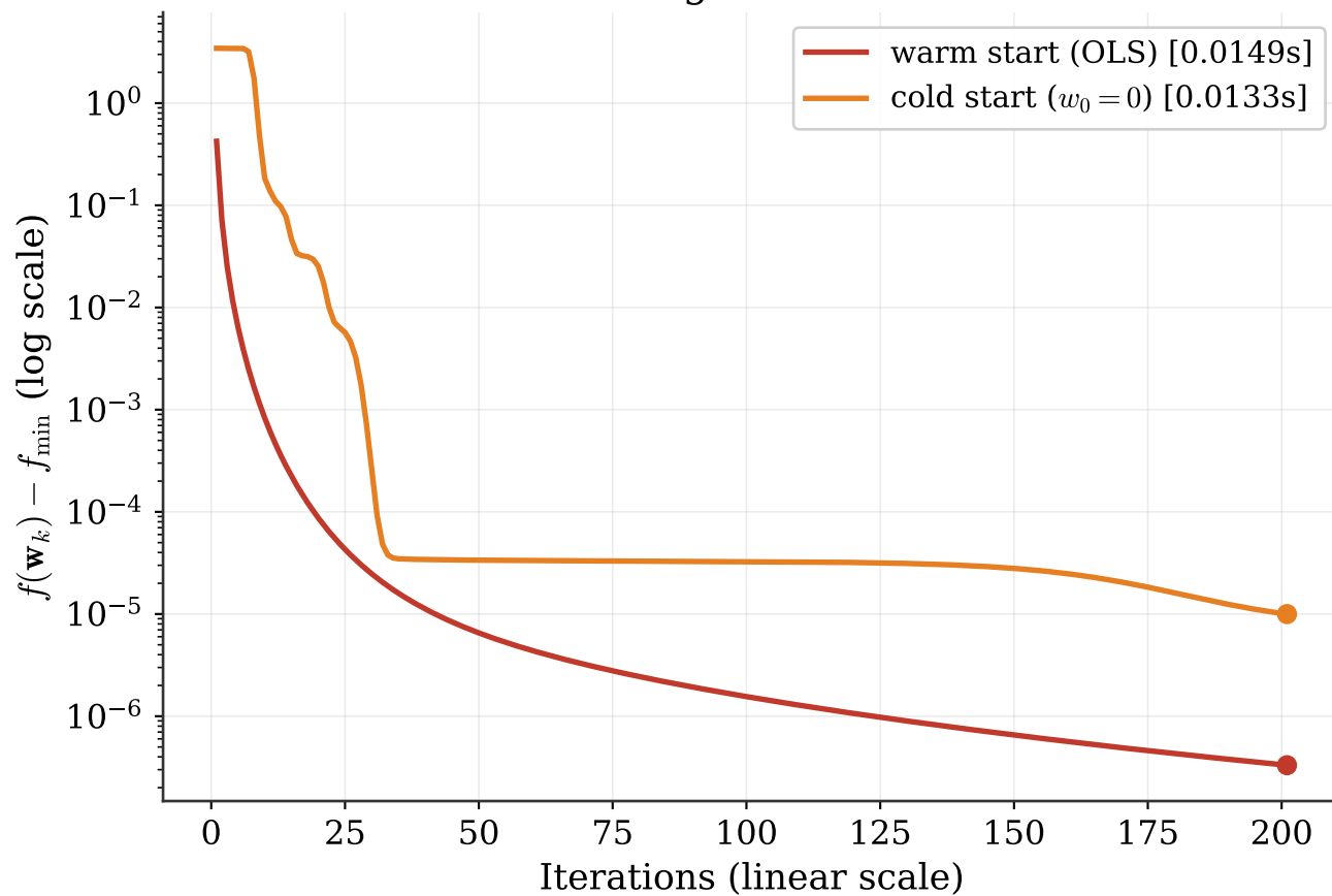
IRLS convergence vs iterations
