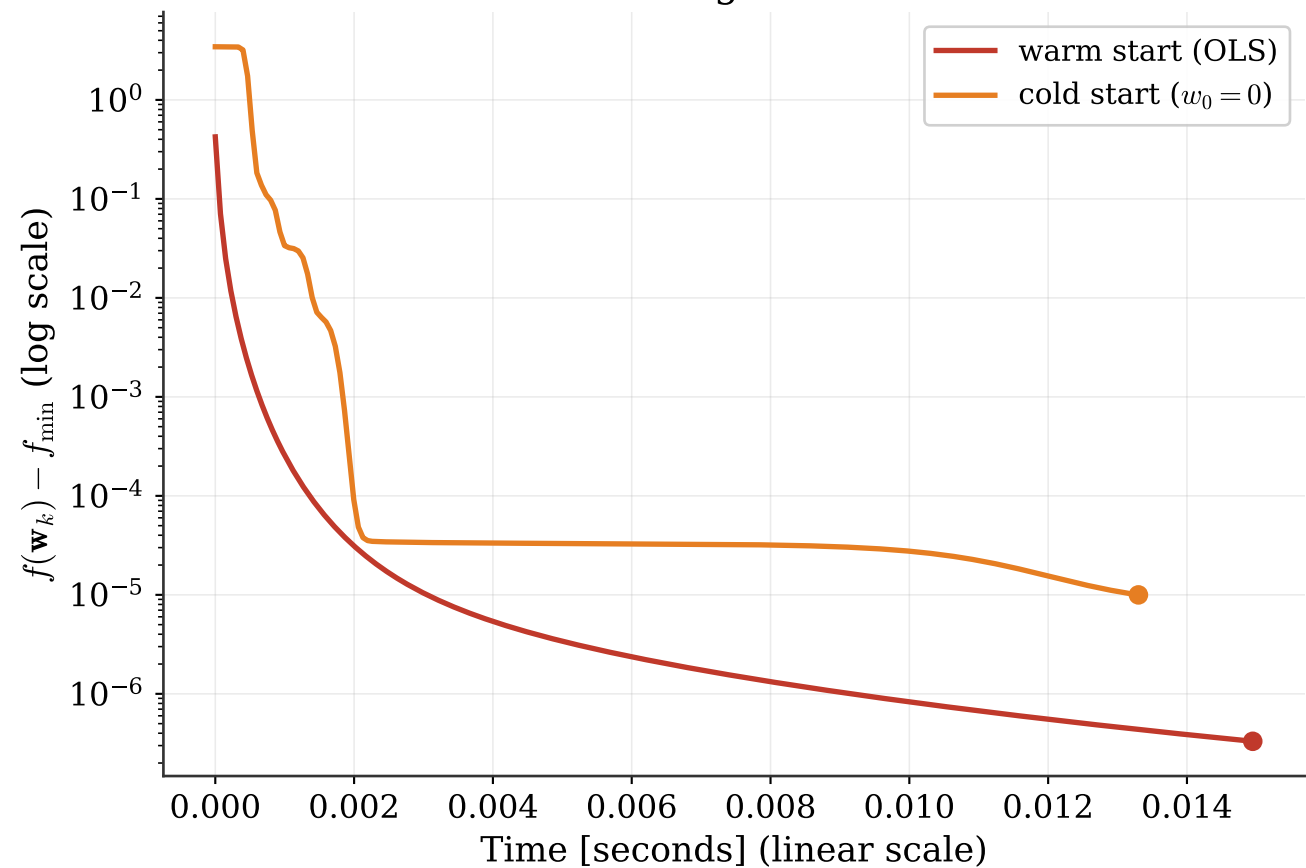
IRLS convergence vs Time
