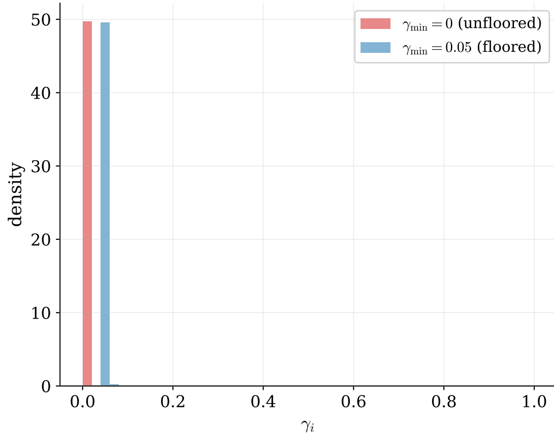
Distribution of \gamma_i over iterations
