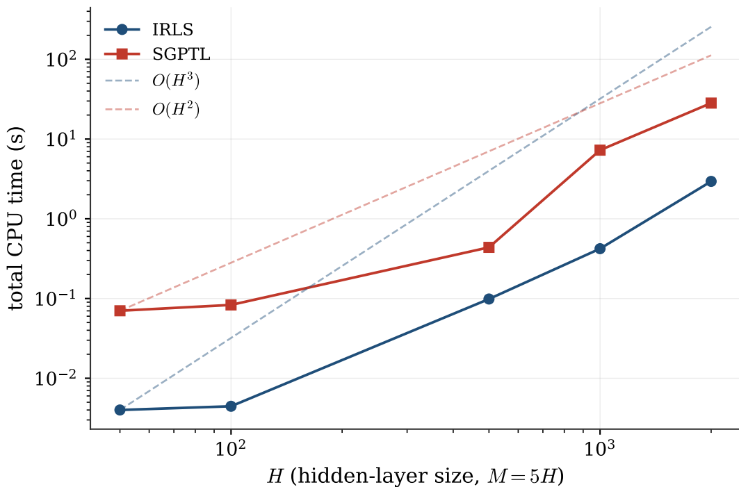
Total time
