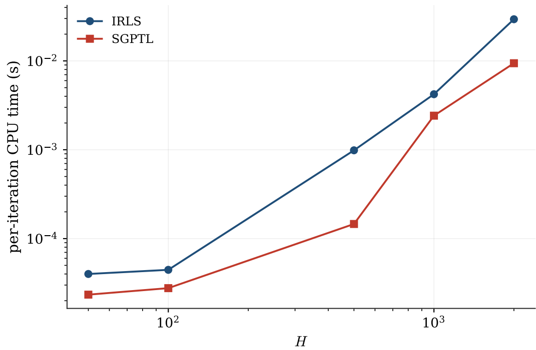
Per-iteration cost
