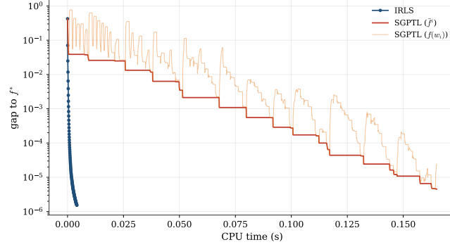
Figure 5.2: Optimality gap versus CPU time on the same instance as Figure 5.1.
