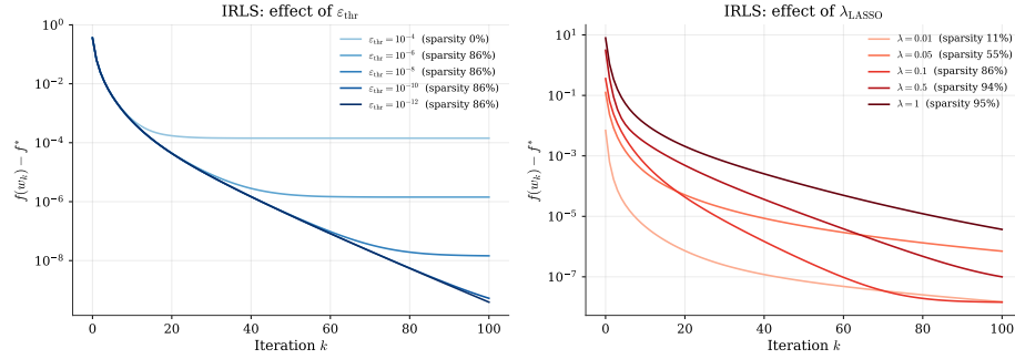
Figure 5.4: IRLS sensitivity. Left: effect of \varepsilon_{\text{thr}} on convergence and sparsity at \lambda_{\text{LASSO}} = 0.1 . Right: effect of \lambda_{\text{LASSO}} at \varepsilon_{\text{thr}} = 10^{-8} .
