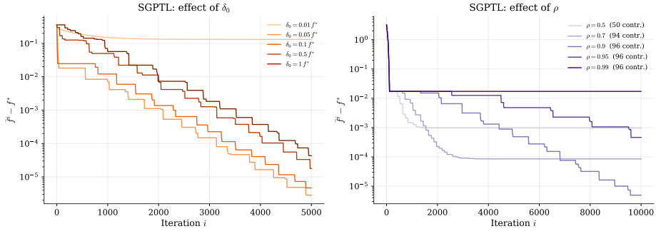
Figure 5.5: SGPTL sensitivity. Left: effect of the initial gap estimate \delta_0 as a fraction of f^* . Right: effect of the contraction factor \rho under a cold start \mathbf{w}_0 = \mathbf{0} (the OLS warm start triggers too few contractions for \rho to matter).
