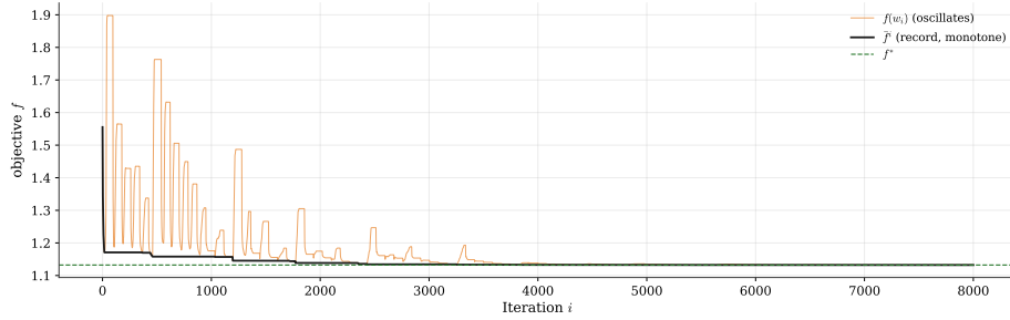
Figure 5.3: SGPTL on the convergence instance. The current value f(\mathbf{w}_i) oscillates while the record value \tilde{f}^i is monotone non-increasing. The dashed green line marks f^* .
