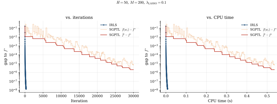
Figure 5.7: IRLS versus SGPTL on the moderate problem. Left: optimality gap versus iteration. Right: gap versus CPU time.
