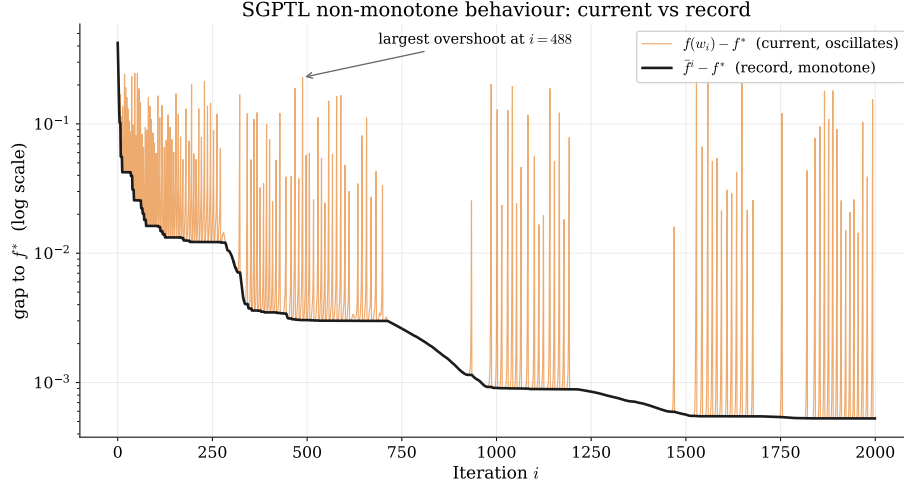
Figure 5.4: SGPTL on the convergence instance, first 2000 iterations, semilog y axis. The current gap f(\mathbf{w}_i) - f^* (orange) spikes well above the record gap f^i - f^* (black) at several points throughout the run, while the record is monotone non-increasing by construction. The largest overshoot is annotated. This is the practical reason why the algorithm returns \mathbf{w}_{\text{best}} rather than the last iterate.
