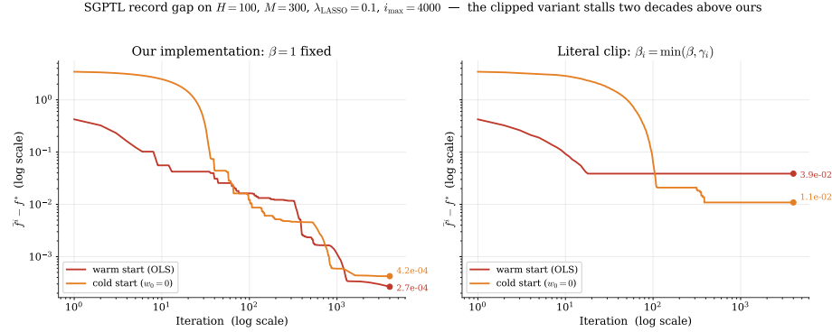
Figure 5.1: SGPTL record gap on H = 100 , M = 300 , \lambda_{\text{LASSO}} = 0.1 , i_{\text{max}} = 4000 , log-log axes, shared y -scale. Left panel: our implementation, \beta = 1 fixed. Right panel: literal clipped reading \beta_i = \min(\beta, \gamma_i) from [10]. Each panel overlays the warm and cold starts; the marker on the right end of each trace annotates the final record gap. Under the clip the iterate freezes within \sim 100 iterations and the gap plateaus at \sim 10^{-2} regardless of starting point ( 3.9 \cdot 10^{-2} warm, 1.1 \cdot 10^{-2} cold). With \beta held fixed the target-level mechanism keeps the iterate moving and the gap descends two to three decades further inside the same budget ( 2.7 \cdot 10^{-4} warm, 4.2 \cdot 10^{-4} cold). The algorithmic choice between clipped and fixed dominates the choice of starting point.
