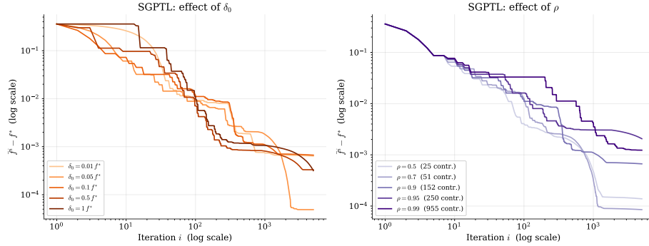
Figure 5.7: SGPTL sensitivity ( H = 100 , M = 400 , OLS warm start, 5000 iterations). Left: effect of \delta_0 as a fraction of f^* at \rho = 0.9 — final gaps cluster in [5 \cdot 10^{-5}, 7 \cdot 10^{-4}] , the algorithm is robust to \delta_0 . Right: effect of \rho at \delta_0 = 0.1 f^* ; aggressive contraction ( \rho = 0.7 ) reaches 8.5 \cdot 10^{-5} , slow contraction ( \rho = 0.99 ) plateaus at 1.2 \cdot 10^{-3} . The contraction count is reported in each legend.
