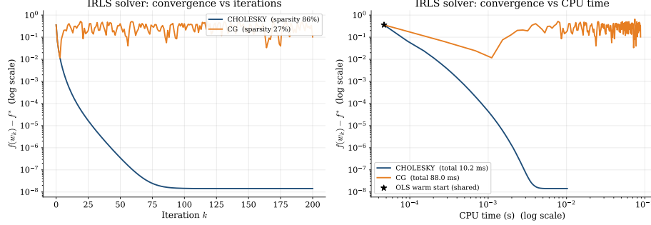
Figure 5.6: IRLS inner-solver comparison on H = 100 , M = 400 , \lambda_{\text{LASSO}} = 0.1 , \varepsilon_{\text{thr}} = 10^{-8} , k_{\text{max}} = 200 . Left: gap f(\mathbf{w}_k) - f^* versus iteration on a semilog y axis. Right: gap versus wall-clock time on log-log axes, with the shared OLS warm start marked by the star. Cholesky descends smoothly to \sim 10^{-8} ( \sim \varepsilon_{\text{thr}} ) within \sim 10 ms; CG oscillates around 10^{-1} for the entire \sim 88 ms budget, never recovering sparsity or a low optimality gap.
