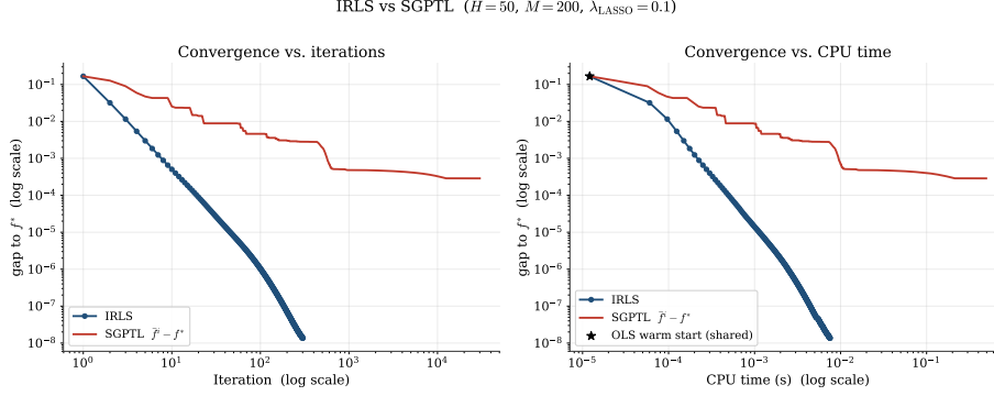
Figure 5.9: IRLS versus SGPTL on the moderate problem ( H = 50 , M = 200 , \lambda_{\text{LASSO}} = 0.1 ). Both panels use log–log axes: linear scaling would crush IRLS’ \sim 100 iterations against the axis next to SGPTL’s 30000. Left: optimality gap versus iteration. Right: gap versus CPU time. SGPTL falls below 10^{-2} in 22 iterations and 10^{-3} in 564, then enters the sublinear regime; IRLS reaches 10^{-8} within \sim 10 ms.
