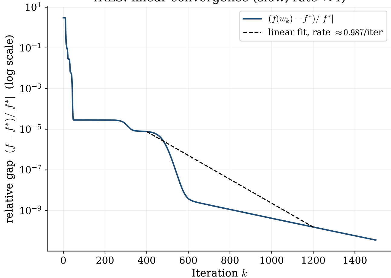
IRLS: linear convergence (slow, rate \approx 1 )
