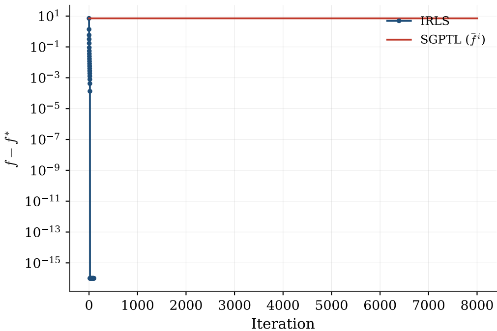
diabetes (M=354, H=200)
