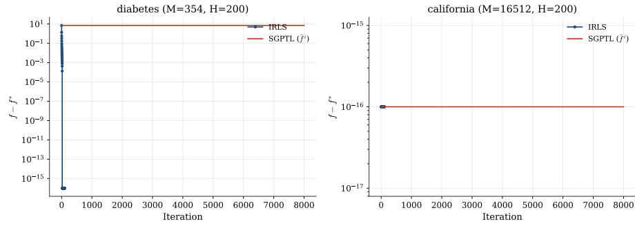
Figure 5.8: Optimisation gap f - f^* versus iteration on the two real datasets. IRLS reaches the sklearn precision floor on both instances; SGPTL converges only on California, where M \gg H keeps the problem well-posed.
