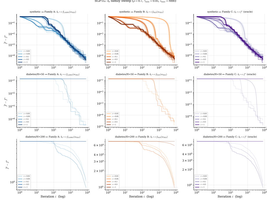
Figure 5.8: Sensitivity of the final record gap to the choice of \delta_0 , three families across three instances: synthetic LASSO ( H = 100, M = 300 , top row, 5 seeds with per-seed thin traces and aggregate-mean thick), diabetes H = 50 (middle, single seed, CVXPY-verified f^* ), diabetes H = 200 (bottom, pre-converged regime). All runs use \rho = 0.7, \gamma_{\min} = 0.05, i_{\max} = 8000 . Family A: \delta_0 = c f_{\text{LASSO}}(\mathbf{w}_{\text{OLS}}) (default, admissible). Family B: \delta_0 = c \frac{1}{2} \|\mathbf{X}\mathbf{w}_{\text{OLS}} - \mathbf{y}\|^2 (admissible). Family C: \delta_0 = c f^* (diagnostic oracle, not admissible). Across all instances and all c in the regime where SGPTL admits progress, Families A and C agree within a factor of 2; at over-aggressive c both families stall at the same plateau and the comparison is uninformative.
