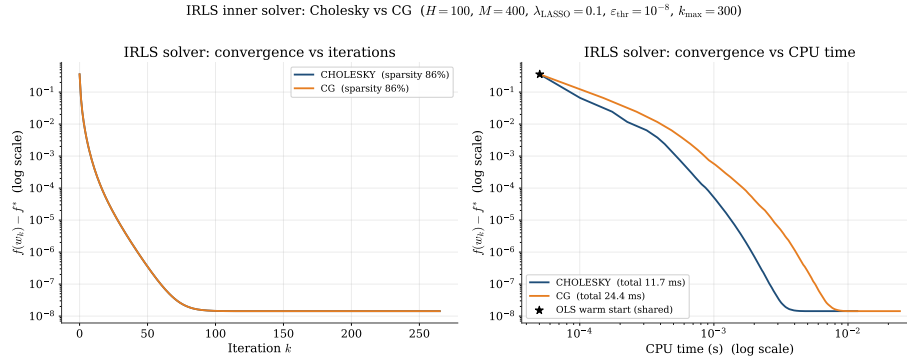
Figure 5.7: IRLS inner-solver comparison on H = 100 , M = 400 , \lambda_{\text{LASSO}} = 0.1 , \varepsilon_{\text{thr}} = 10^{-8} , k_{\text{max}} = 300 . Left: gap f(w_k) - f^* versus iteration on a semilog y axis. Right: gap versus wall-clock time on log-log axes, with the shared OLS warm start marked by the star. Cholesky descends smoothly to \sim 10^{-8} ( \sim \varepsilon_{\text{thr}} ) within \sim 11.7 ms; CG achieves the exact same iterations trajectory but requires \sim 24.4 ms.
