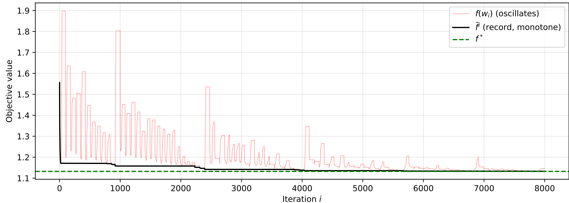
DSM — Non-monotone iterates vs monotone record
