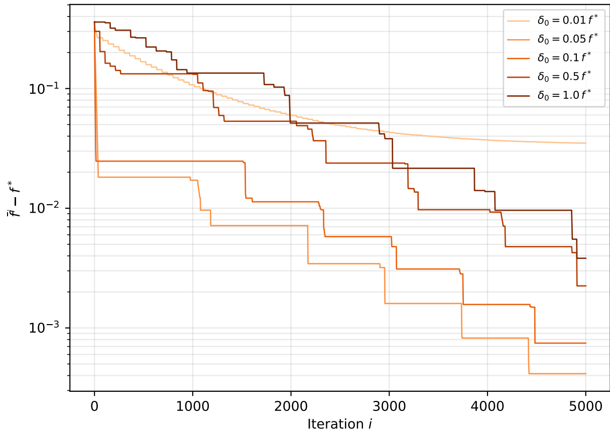
DSM: effect of \delta_0
