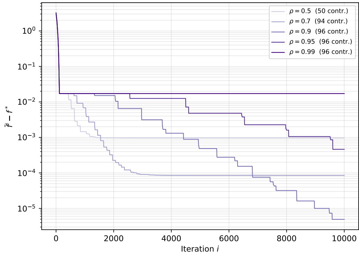
DSM: effect of \rho
