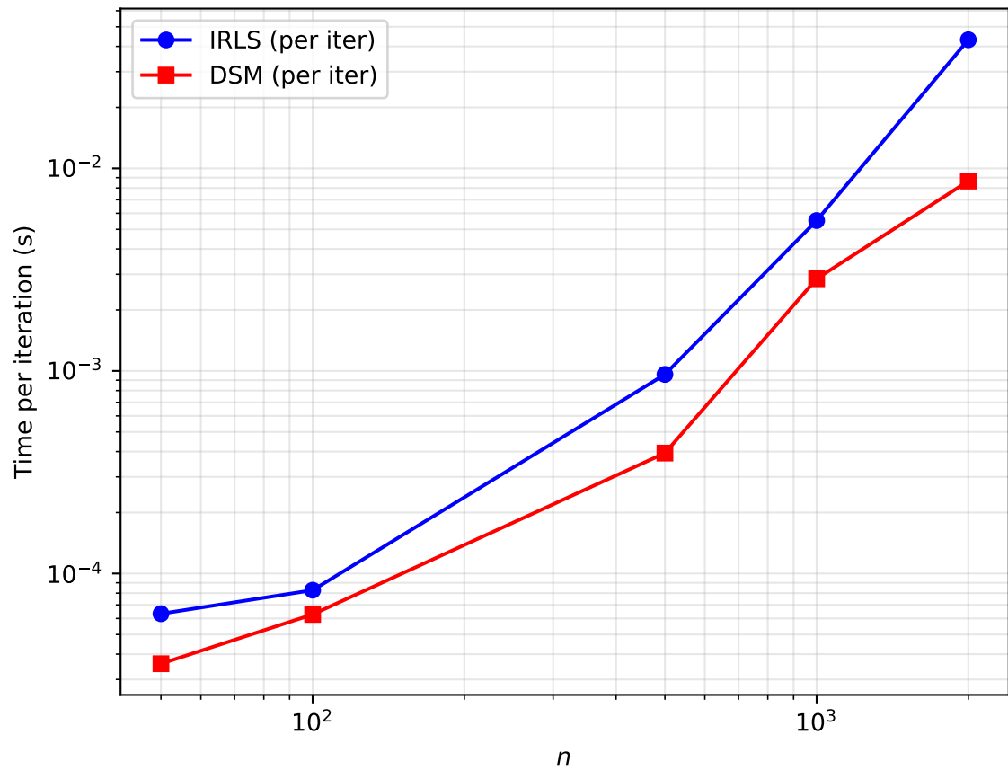
Per-iteration cost
