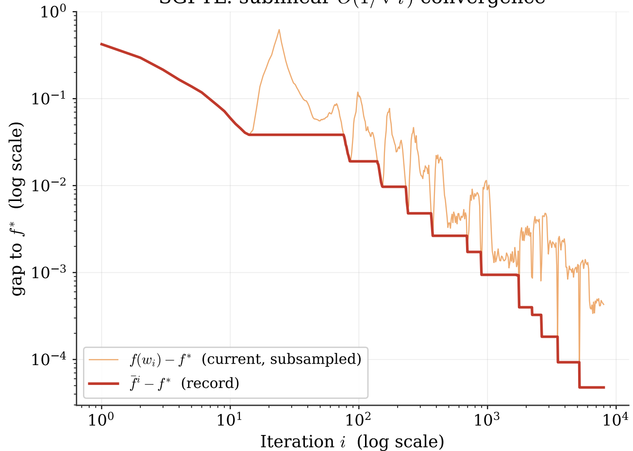
SGPTL: sublinear O(1/\sqrt{i}) convergence
