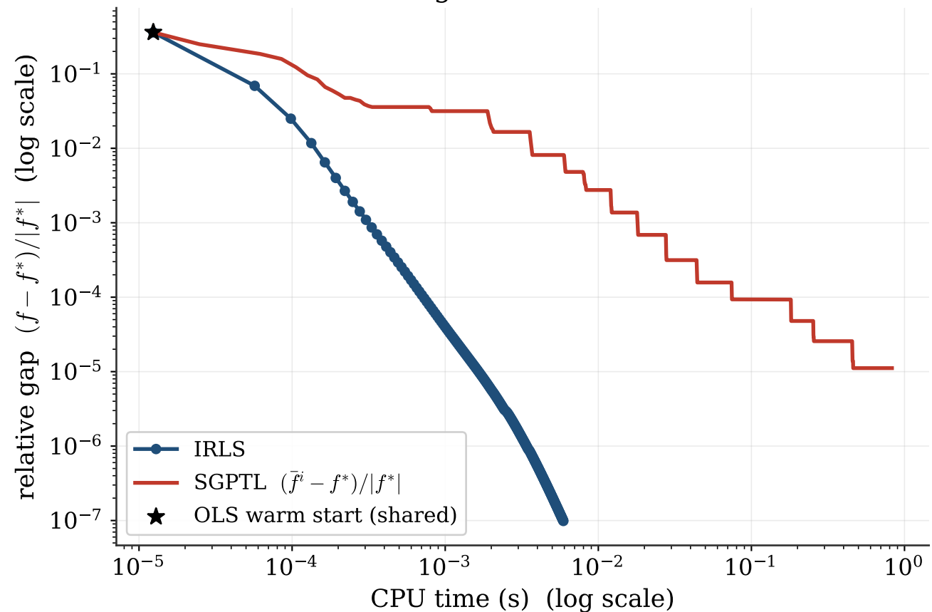
Convergence vs. CPU time
