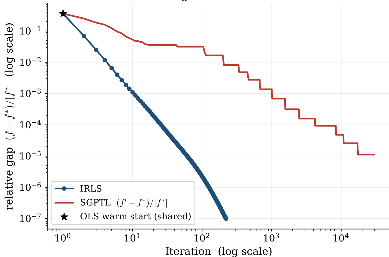
Convergence vs. iterations
