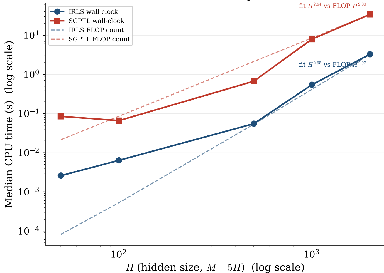
FLOP count vs wall-clock (synthetic, M=5H )
