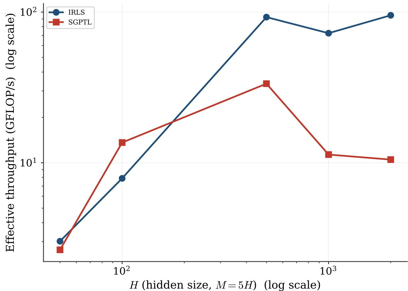
FLOP / wall-clock
