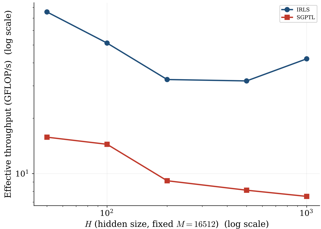
FLOP / wall-clock
