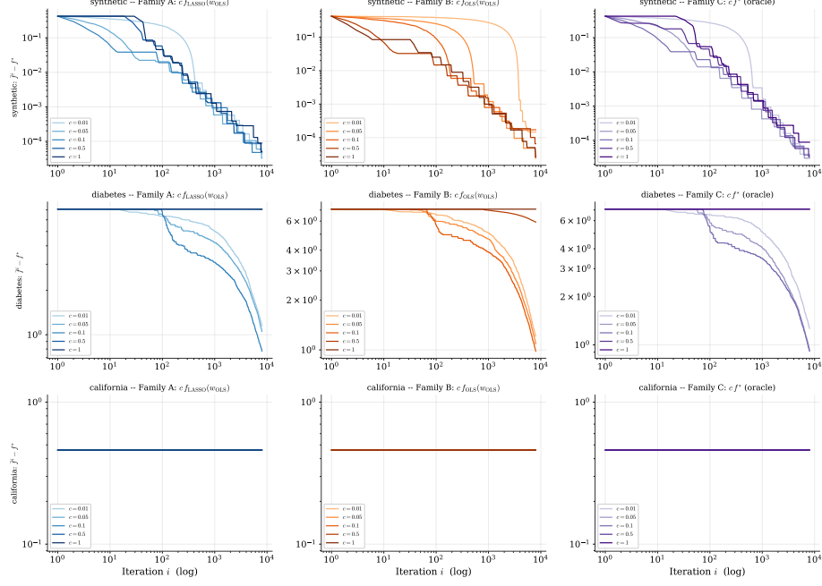
Figure 5.8: Sensitivity of the final record gap to the choice of \delta_0 , three families across three instances: synthetic ( H = 100 , M = 300 , top row), diabetes (middle), and california (bottom), each with \rho = 0.7 , \gamma_{\min} = 0.05 , i_{\max} = 8000 . Family A: \delta_0 = c f_{LASSO}(w_{OLS}) (our default, admissible); Family B: \delta_0 = c \frac{1}{2} \|\mathbf{X}w_{OLS} - \mathbf{y}\|^2 (admissible); Family C: \delta_0 = c f^* (diagnostic oracle on synthetic; IRLS-converged proxy on real data; never used in reported runs). Each panel sweeps c \in \{0.01, 0.05, 0.1, 0.5, 1\} . Families A and C overlap on synthetic within a factor of three, on diabetes within 15%, and on california to four digits.
