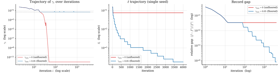
Figure 5.8: Floor test on ELM LASSO ( H = 100 , M = 300 , \lambda_{\text{LASSO}} = 0.1 , i_{\max} = 4000 , \rho = 0.7 ), single seed shown. Left: trajectory of \gamma_i over the run (log-log). Without the floor, \gamma_i collapses below 10^{-10} around iteration 50 and stays there; with \gamma_{\min} = 0.05 it sits on the floor (dotted grey line) for the rest of the run. Centre: target gap \delta_i ; the unfloored \delta contracts twice and stops, the floored one descends in the staircase the theory expects. Right: record relative gap (\bar{f}^i - f^*)/|f^*| ; the floor buys two orders of magnitude. The aggregate over the 30 runs of the binary grid agrees with this single-seed snapshot.
