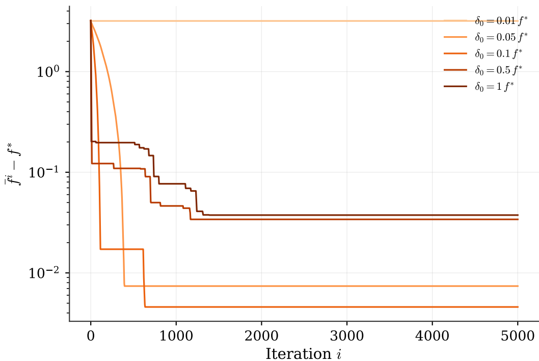
SGPTL: effect of \delta_0
