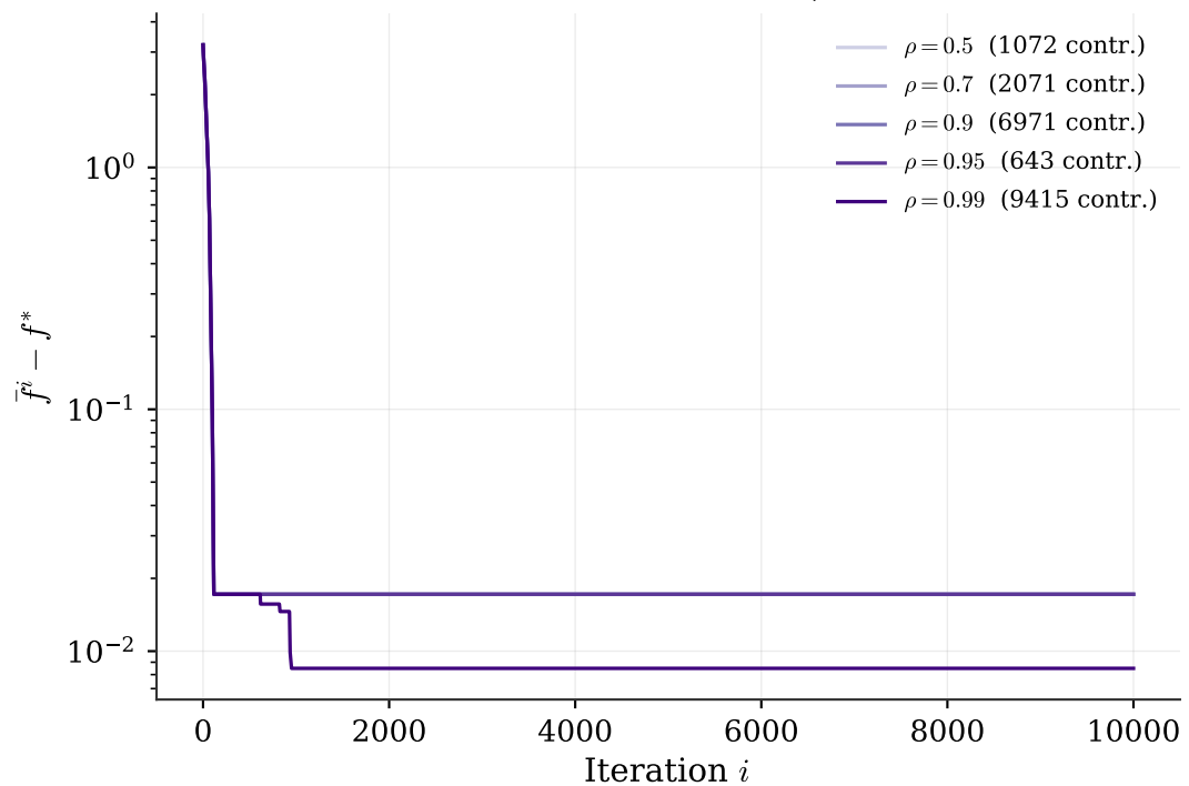
SGPTL: effect of \rho
