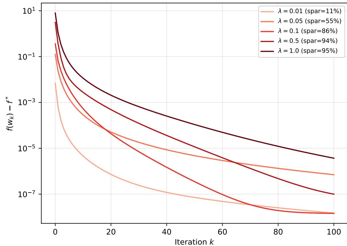
IRLS: effect of \lambda
