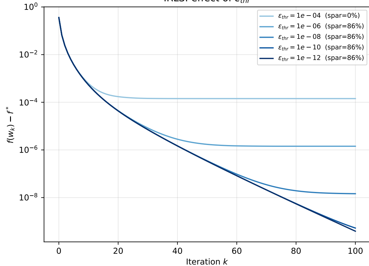
IRLS: effect of \varepsilon_{thr}
