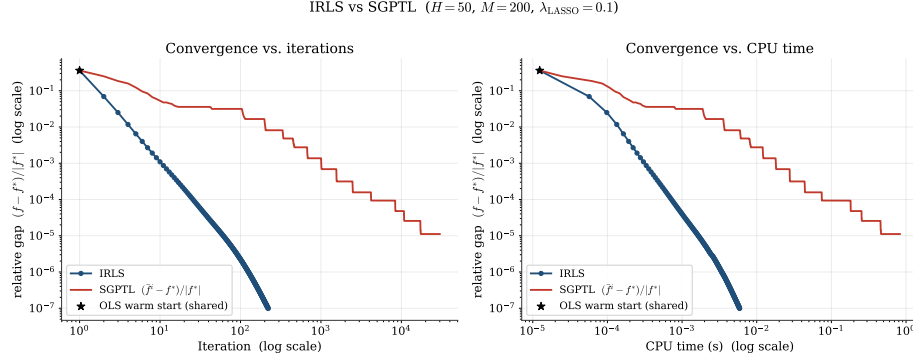
Figure 5.12: IRLS vs SGPTL on H = 50 , M = 200 , \lambda_{\text{LASSO}} = 0.1 , log-log, relative gap (f - f^*)/|f^*| . Left: vs iteration. Right: vs CPU time. SGPTL falls below 10^{-2} in 203 iterations and 10^{-3} in 1008 then enters the sublinear regime; IRLS reaches 10^{-6} in 125 iterations ( \sim 3 ms).
