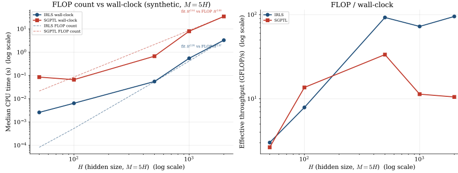
Figure 5.10: Synthetic regime ( M = 5H ). Left: median wall-clock (solid) and analytic FLOP count (dashed, anchored on the largest- H point), log-log, with fitted slopes annotated. Right: effective throughput, FLOP count divided by wall-clock. IRLS rises toward the BLAS peak; SGPTL throughput drops near H = 1000 , where the working set exceeds cache.
