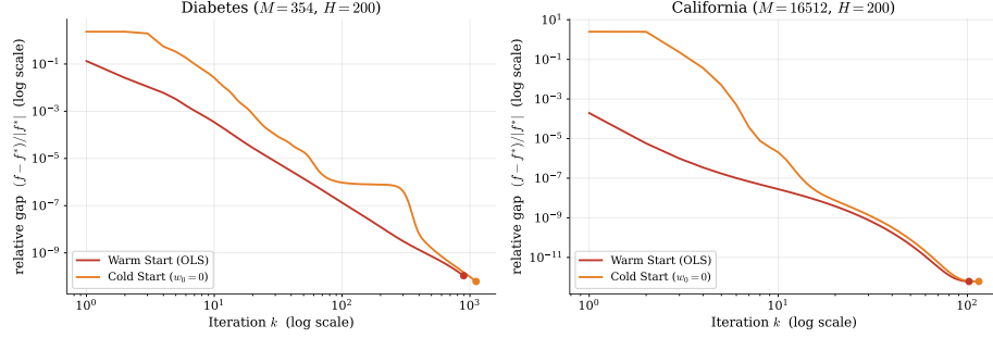
Figure 5.4: IRLS warm (OLS) vs cold ( \mathbf{w}_0 = \mathbf{0} ) start on the two ELM-transformed real datasets ( H = 200 , \lambda_{\text{LASSO}} = 0.1 , k_{\text{max}} = 2000 , \varepsilon_{\text{thr}} = 10^{-8} , \varepsilon_{\text{stop}} = 10^{-8} ), log-log axes, relative gap (f - f^*)/|f^*| measured against an independent reference f^* (a separate deeper IRLS run at \varepsilon_{\text{thr}} = 10^{-14} , cross-validated against CVXPY-Clarabel, Section 5.6). Both starts descend to the O(\varepsilon_{\text{thr}}) smoothing floor of the displayed runs; the warm curve sits below the cold one throughout because \|\mathbf{w}_0 - \mathbf{w}^*\| enters the linear-rate bound multiplicatively. The synthetic analogue is in Appendix C.
