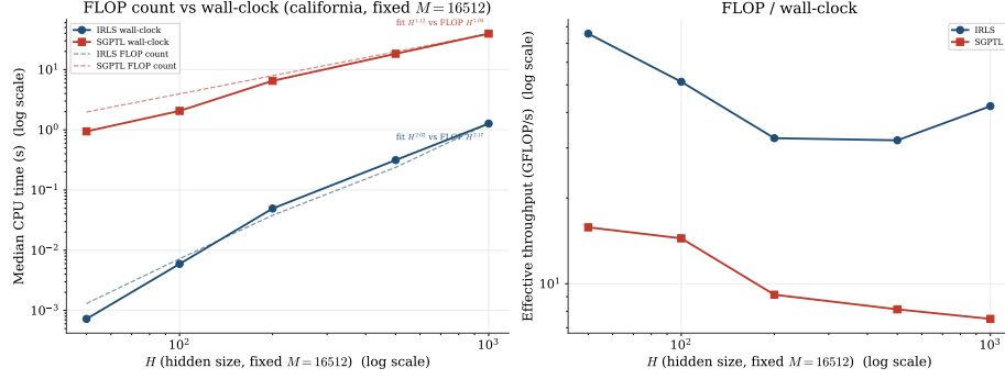
Figure 5.11: Real regime (california, M = 16512 fixed): neuron scaling in H . Left: wall-clock vs FLOP count; right: throughput. With M fixed the FLOP exponents fall to \approx 2 (IRLS) and \approx 1 (SGPTL), and wall-clock tracks them.
