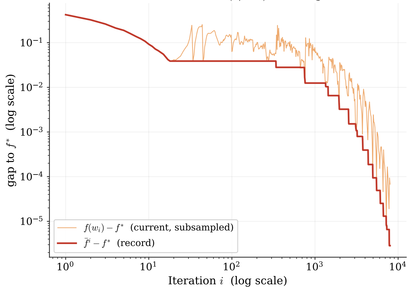
SGPTL: sublinear O(1/\sqrt{i}) convergence
