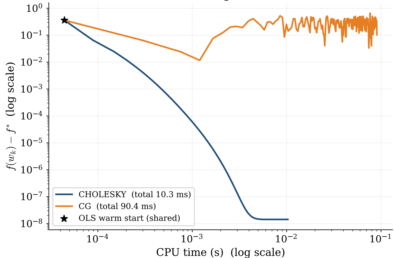
IRLS solver: convergence vs CPU time
