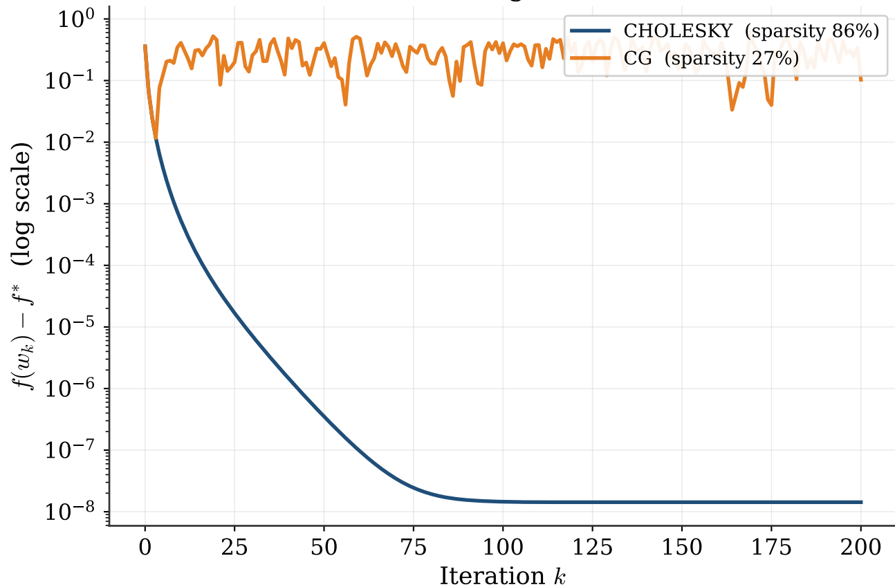
IRLS solver: convergence vs iterations
