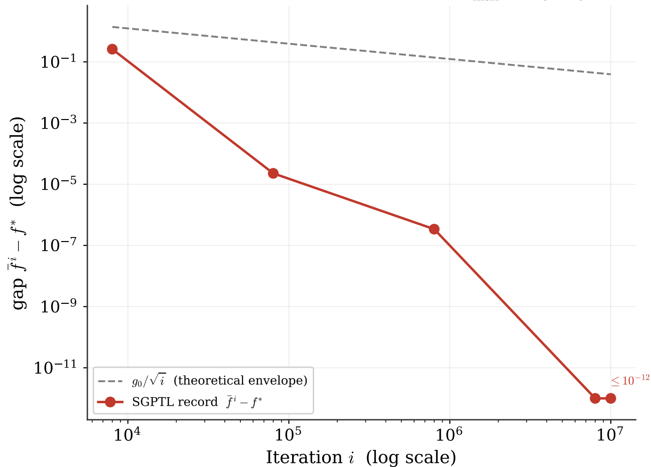
diabetes cold start ( H = 200 , \lambda = 0.1 , i_{\max} = 10,000,000 )
