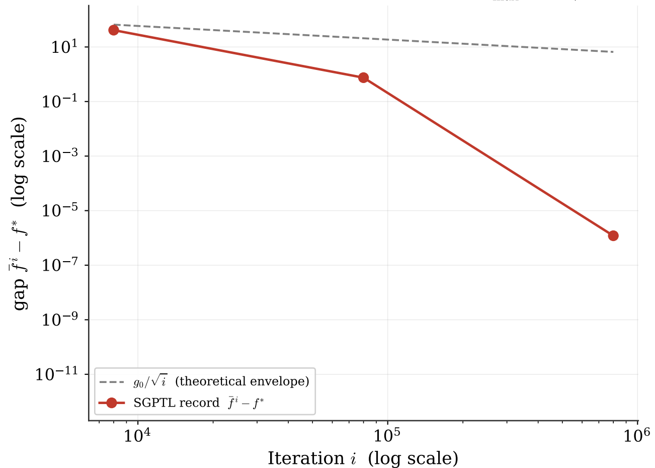
california cold start ( H = 200 , \lambda = 0.1 , i_{\max} = 800,000 )
